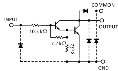
ULN2004APG/AFWG
